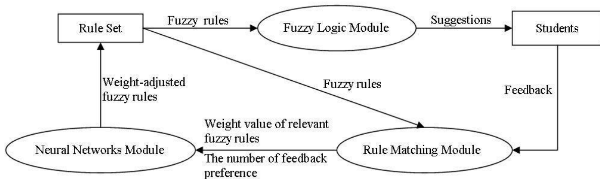
Figure 3: The execution phase to adjust rule weight.
