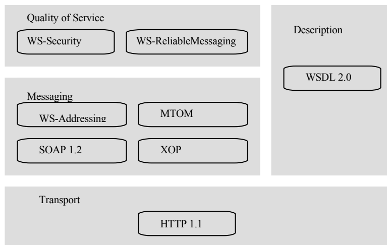
Figure 2: NEHTAs recommended Web Services standards Model
