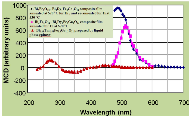
Fig.3. Measured spectral dependencies of MCD signal in (◆) RF co-sputtered ( \text{Bi}_3\text{Fe}_5\text{O}_{12} - \text{Bi}_2\text{Dy}_1\text{Fe}_4\text{Ga}_1\text{O}_{12} ) composite film of thickness about 1 \mu\text{m} , annealed for 1 hour at 520 ^{\circ}\text{C} at first stage and later re-annealed for 1 hour at 530 ^{\circ}\text{C} ; (■) co-sputtered composite film of the same stoichiometry when still mainly in its amorphous phase and of the same thickness, but only annealed for 1 hour at 520 ^{\circ}\text{C} ; and (▲) \text{Bi}_{0.45}\text{Tm}_{2.55}\text{Fe}_{3.8}\text{Ga}_{1.2}\text{O}_{12} film prepared by LPE. Sensitivity scale of the dichrometer was the same during all measurements.
