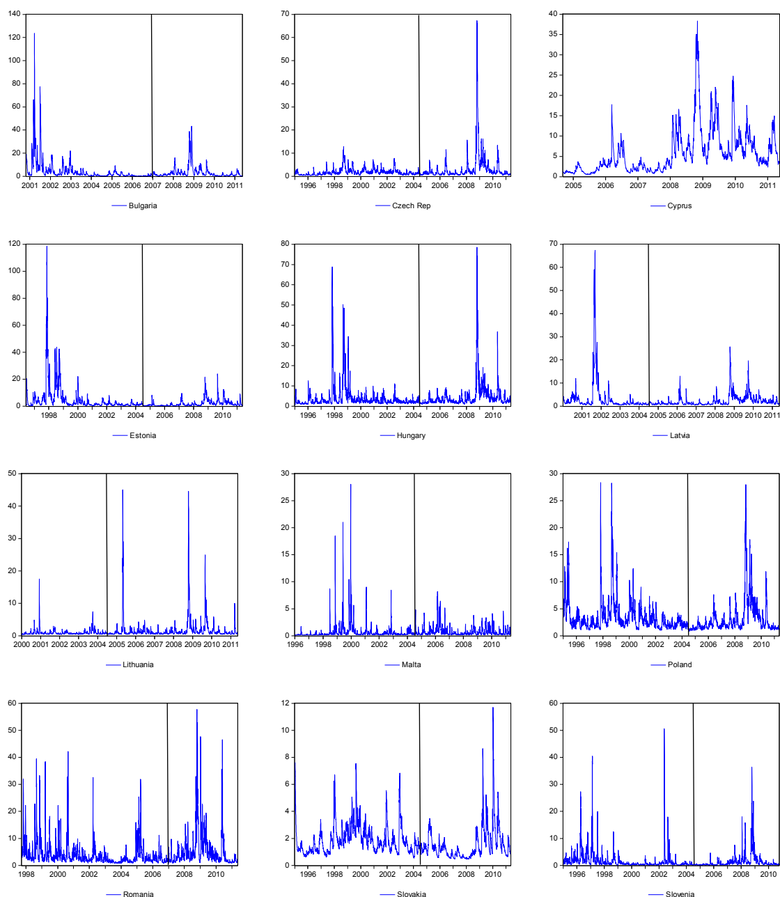
Figure I. 1: Conditional variances of GARCH (1,1) model
