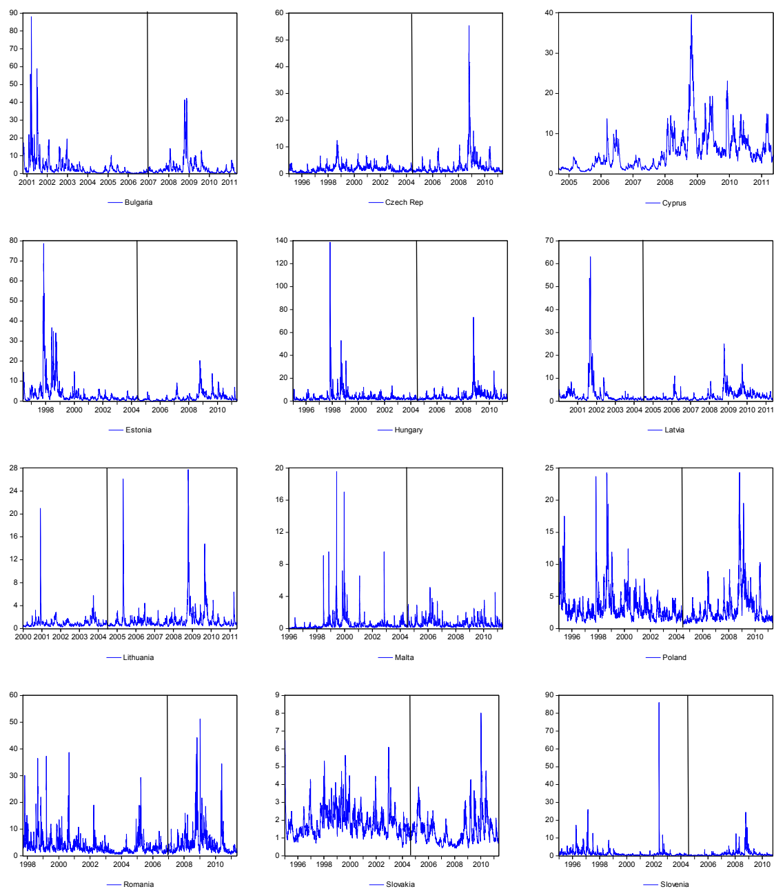
Figure I.2: Conditional variances of EGARCH model
