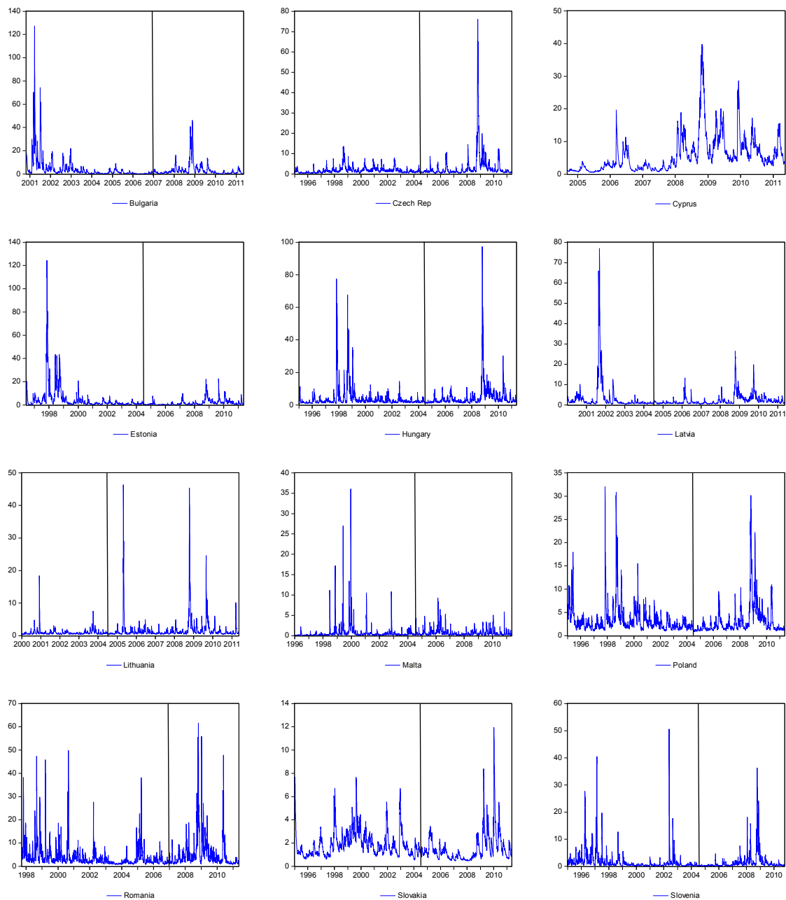
Figure I.3: Conditional variances of GJR model
