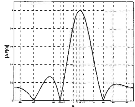
Fig. 4. The simulated azimuth gain patter of 4-element Array Factor for the proposed photonic null steering antenna array.
