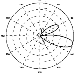
Fig. 5. Polar plot of 4-element antenna pattern with desired signal (main lobe) at -15^\circ and interfering signals (nulls) at -60^\circ , -20^\circ and 80^\circ .
