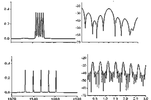
Fig. 6. Optical spectrum of RF-modulated wavebands (left) and measured RF responses for different waveband spacing scenarios
