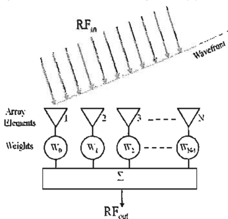
Fig. 1. Generic N-element antenna array structure.
