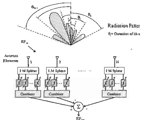
Fig. 2. Phased-array antenna structure for broadband null steering.
