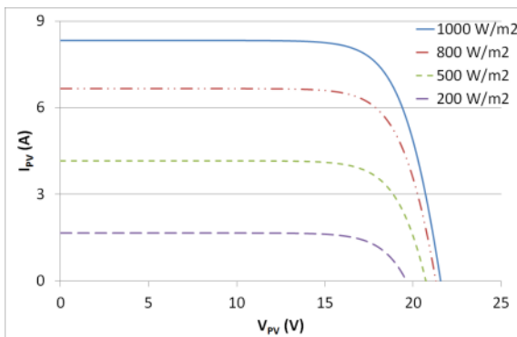
Figure 4 - Modelled PV characteristics: current versus voltage at varying I_G ( T_A=25^\circ\text{C} , W_S=0\text{m/s} ).
