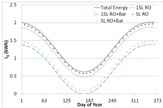
Figure 12- Excess energy available after RO and battery charging for A_{PV}=2.6\text{m}^2 (circles: 5L/day RO; dashed lines for 15L/day RO)
