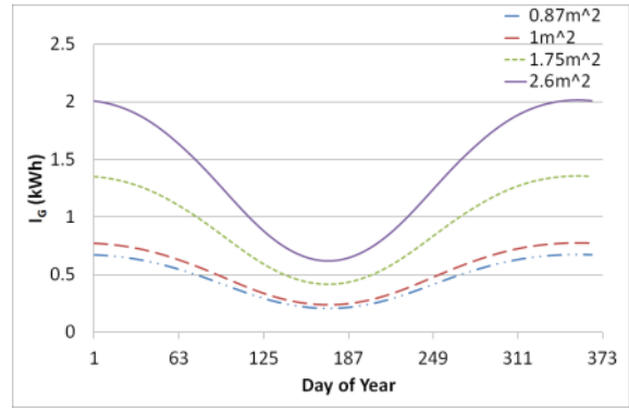
Figure 11- Solar energy available at varying PV panel area (1 panel area A_{PV}=0.87\text{m}^2 , 2 panels A_{PV}=1.75 and 3 panels A_{PV}=2.6\text{m}^2 ).
