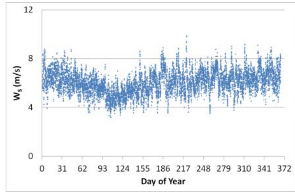
Figure 7- Annual variation of wind speed for a Perth based location (data: BOM, 2011c).
