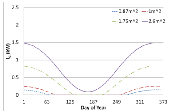
Figure 13- Excess energy available at varying A_{PV} (5L/day RO and battery charge to \text{SOC}_{\text{BAT}}=100\% ).
