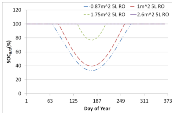
Figure 14- \text{SOC}_{\text{BAT}} at varying A_{PV} for a water production at 5L/day.
