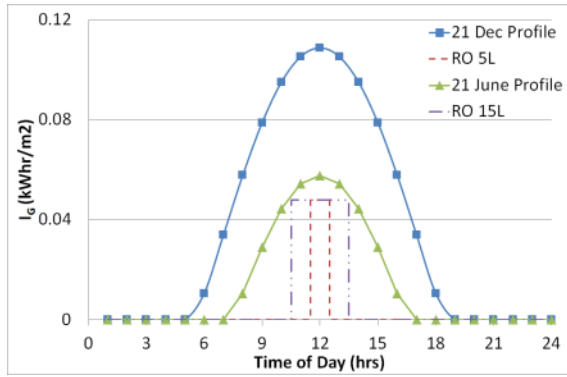
Figure 10- Solar irradiance for the shortest and longest day with energy requirements (kWhr) for desalination of 5L and 15 litres per day.
