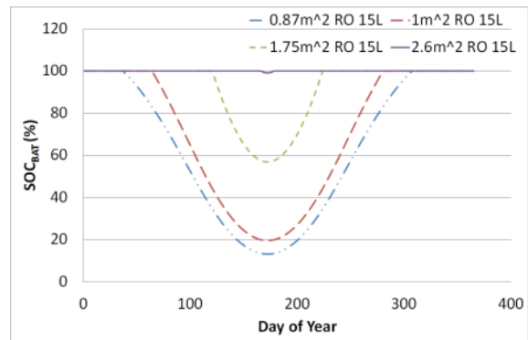
Figure 15- \text{SOC}_{\text{BAT}} at varying A_{PV} for a water production at 15L/day.
