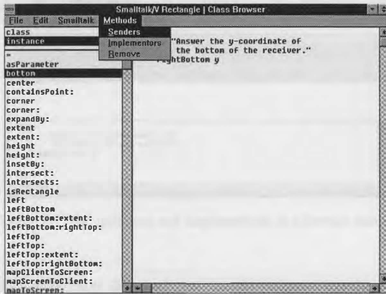
Figure 70. Selecting initiators and implementors of a service method.
