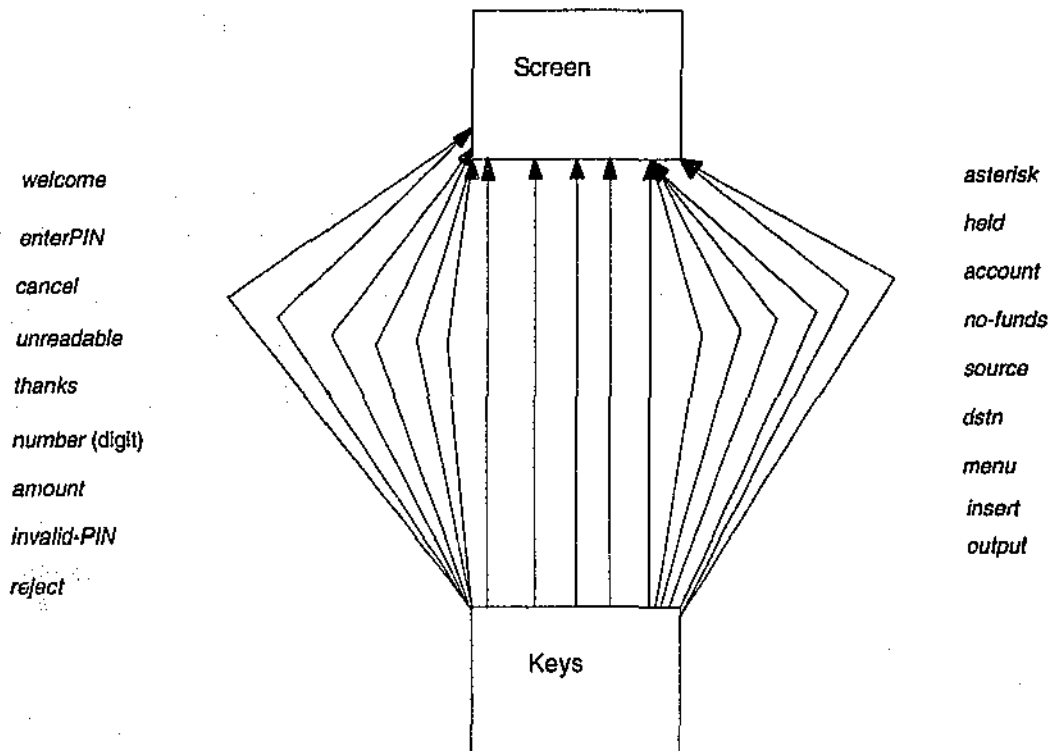
Figure 23. High dependency between objects.
