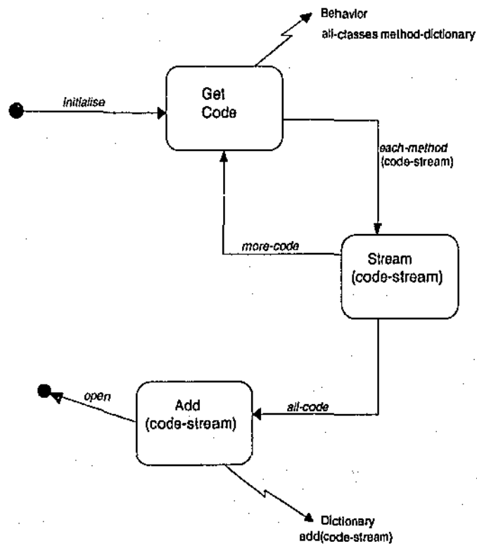
Figure 55. The initialise model for Class Find.
