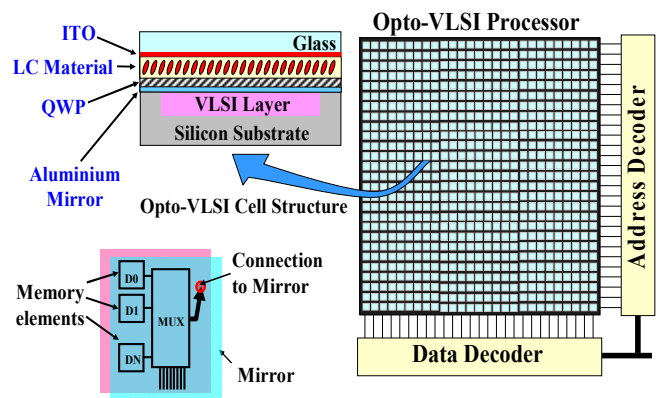
Fig. 1. Opto-VLSI processor structure. By addressing each pixel independently a phase hologram can be synthesized leading to optical beam steering and shaping.
