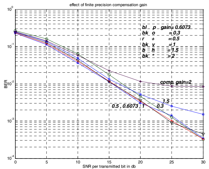
Figure 3. Compensation gain analysis
