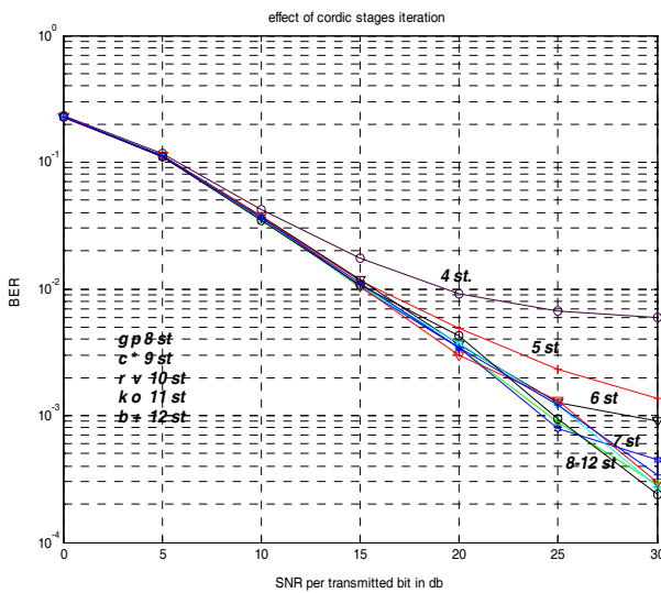
Figure 4. CORDIC iterations analysis
