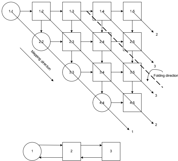
Figure 2. Triangular systolic array
