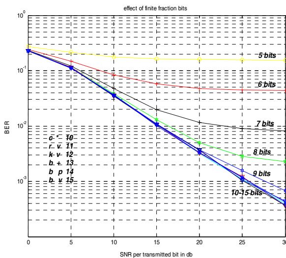
Figure 5 - Finite word length analysis
