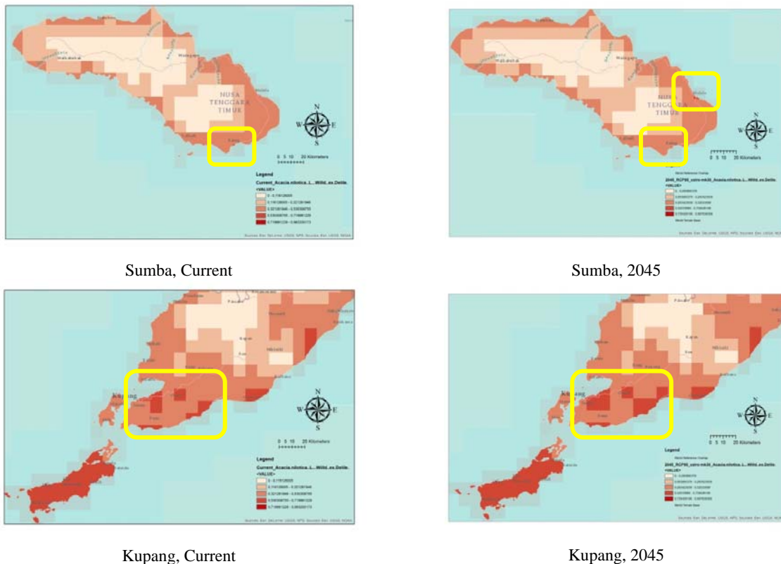
Figure 3. Projection of Acacia nilotica species distribution/Habitat Suitability Index (HSI) on Sumba Island and Kupang, East Nusa Tenggara Province, Indonesia by 2045. Left: Predicted current distribution/current HSI. Right: Projected distribution/projected HSI in 2045. Yellow square to show to emphasize where the HSI changed.
