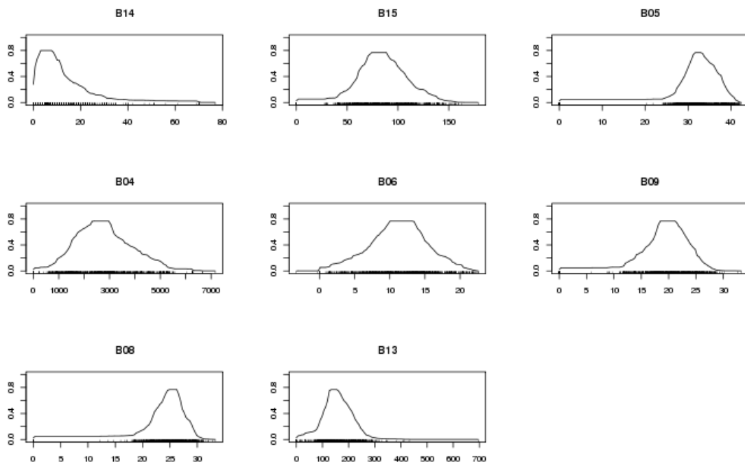
Figure 4. The response curve for Acacia nilotica distribution model. B05 = maximum temperature of warmest month, B06 = minimum temperature of coldest month, B08 = mean temperature of wettest quarter, B09 = mean temperature of driest quarter, B13 = precipitation of wettest month, B14 = precipitation of driest month, B15 = precipitation seasonality and B04 = temperature seasonality
