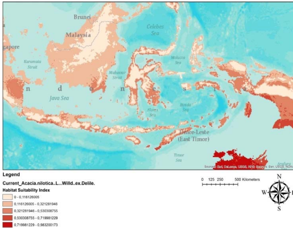
Figure 1. Predicted current distribution (habitat suitability map) of Invasive Alien Species (IAS) Acacia nilotica in Indonesia under current climate condition using Generalized Linear Model (GLM) algorithm in BCCVL. Darker areas representing a higher likelihood that the species can occur. The square yellow line to point out Alas Purwo National Park East Java, Bali, Lombok and Sumba Islands, Kupang NTT Province and West Papua.
