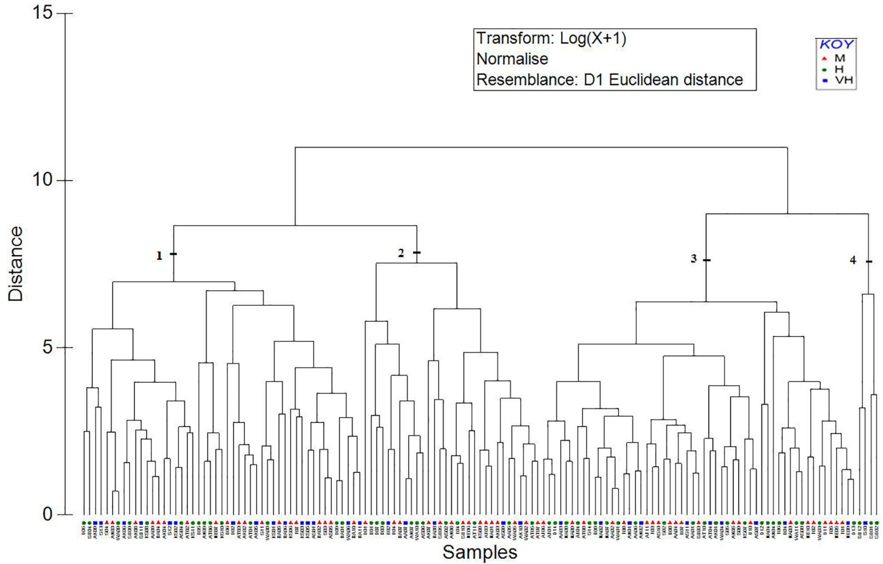
Figure 6. Hierarchical cluster analysis (HCA) of 139 Allanblackia parviflora kernel oil yield (KOY) relationship (M, H and VH) due to tree, fruit and seed morphological characteristics, showing the four clusters at Euclidean distance 7.5.
