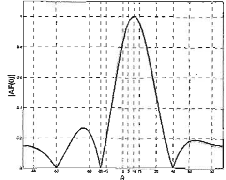
Fig. 4. The simulated azimuth gain pater of 4-element Array Factor for the proposed photonic null steering antenna array.
