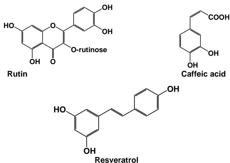
Fig. 1. Chemical structures of common plant derived phenolics (Rutin, Caffeic acid and Resveratrol)
