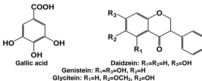
Fig. 3. Chemical structures of common plant derived tannis (Gallic acid, Daidzein, Genistein and Glycitein)
