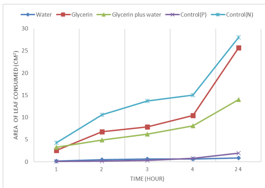
Fig. 6. Rate of leaf consumption by armyworms (cm 2 /hour)
