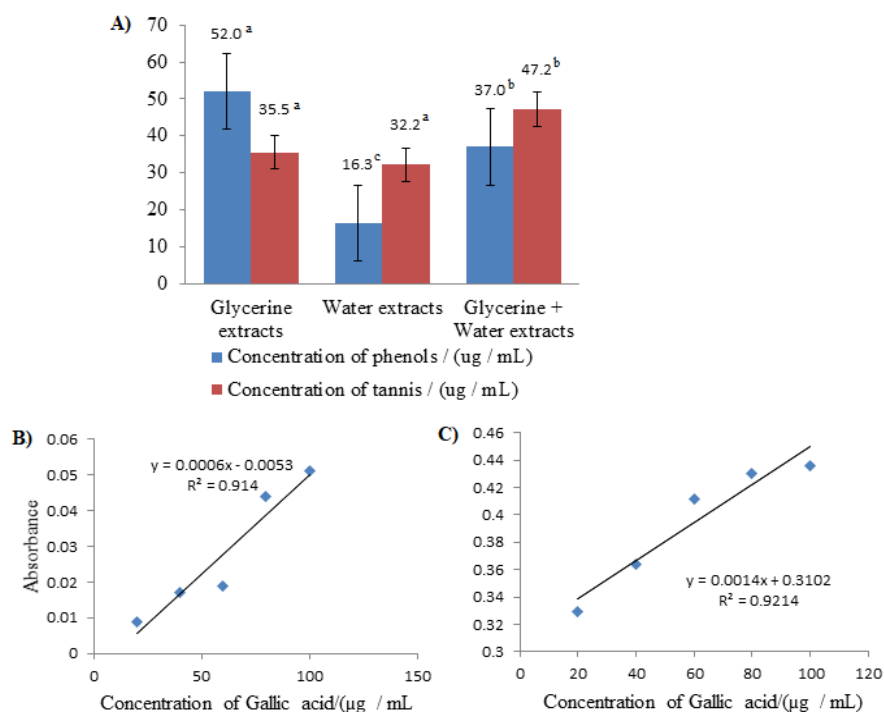
Fig. 5. A) Concentration of phenols and tannins in different aqueous extracts of Mentha spicata . B) Calibration curve of tannins C) Calibration curve for phenols
