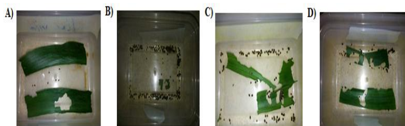
Fig. 7. Observed area of consumption of maize leaves by Spodoptera frugiperda A) Water extracts B) Glycerine extracts C) Glycerine plus water extract D) Control (Neem seed)
