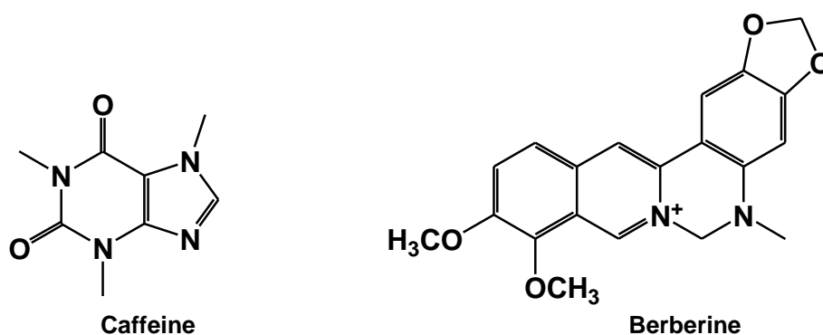
Fig. 2. Chemical structures of common plant derived alkaloids (Caffeine and Berberine)
