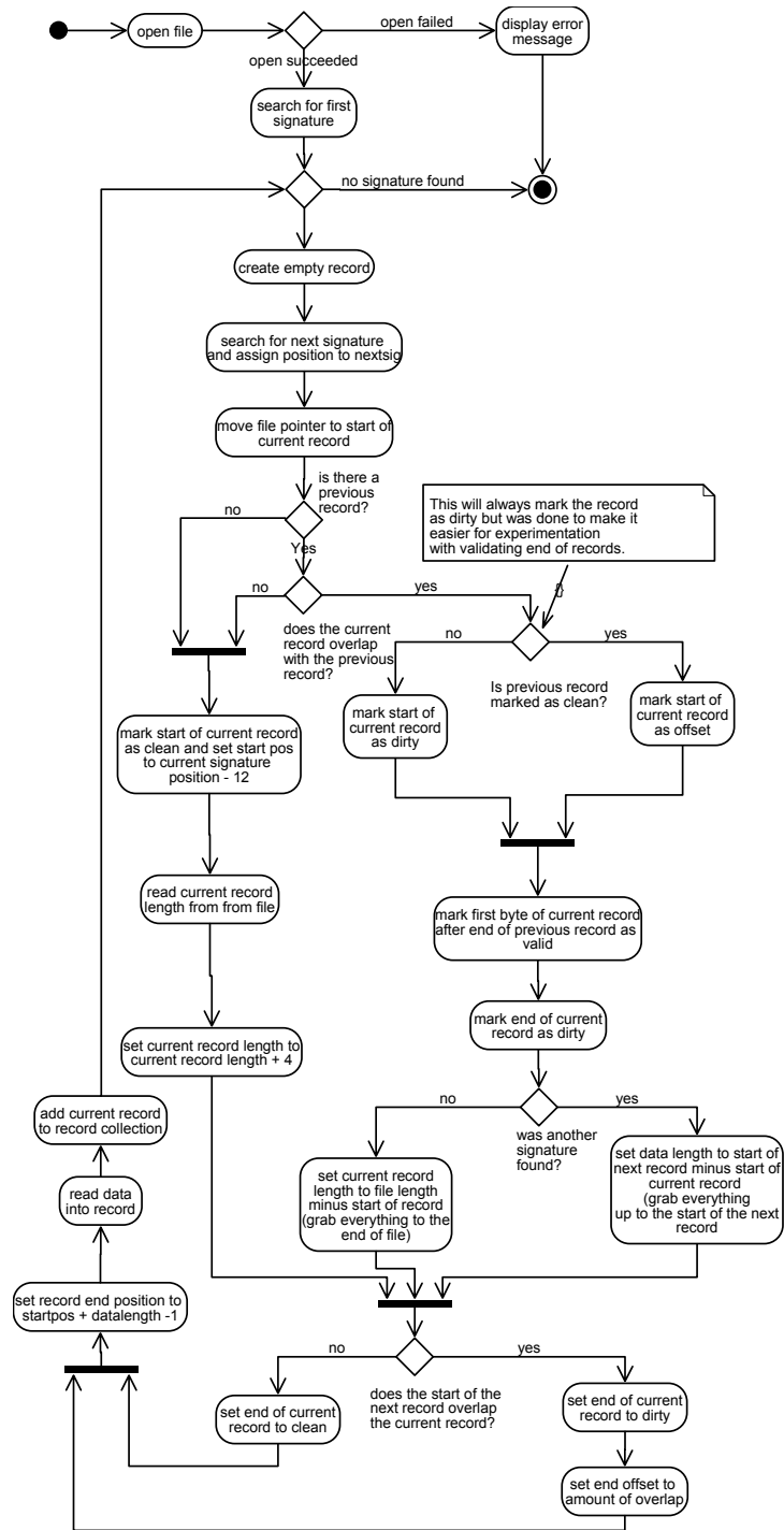
Figure 5: Extraction algorithm
