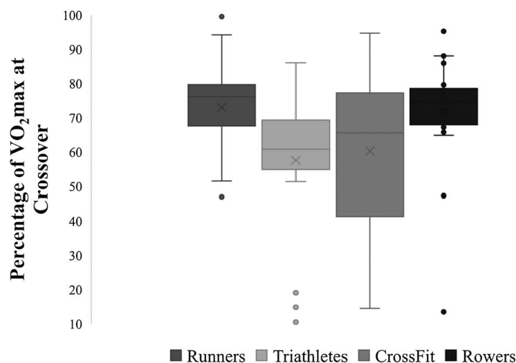
Figure 2: Differences in percentage of \text{VO}_{2\text{max}} at crossover point between sport types. Data points represented by dots indicate outliers within sport group. Triathletes' percent \text{VO}_{2\text{max}} at crossover was significantly lower than runners ( P = 0.04 ) and rowers ( P = 0.04 ).
