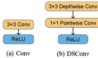
Figure 2: Standard convolution and depthwise separable convolution
