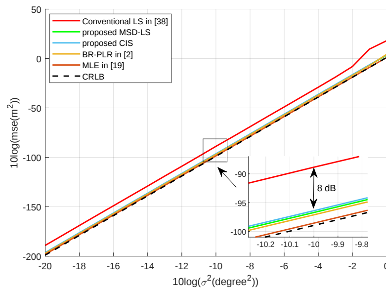
Figure 3. MSE of different AOA localization methods with different angle noise.
