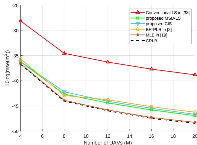
Figure 4. MSE of different AOA localization methods with different numbers of UAVs.
