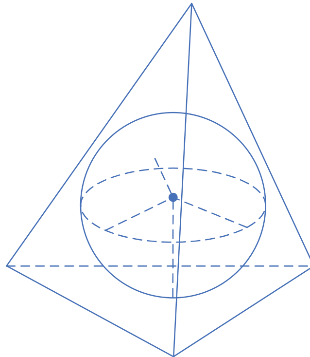
Figure 2. The center of inscribed sphere for a tetrahedron.
