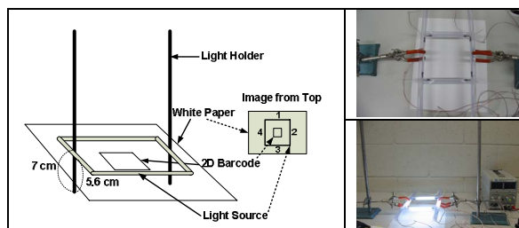
Figure 2. Light setting with top view (above) and front view (below).
