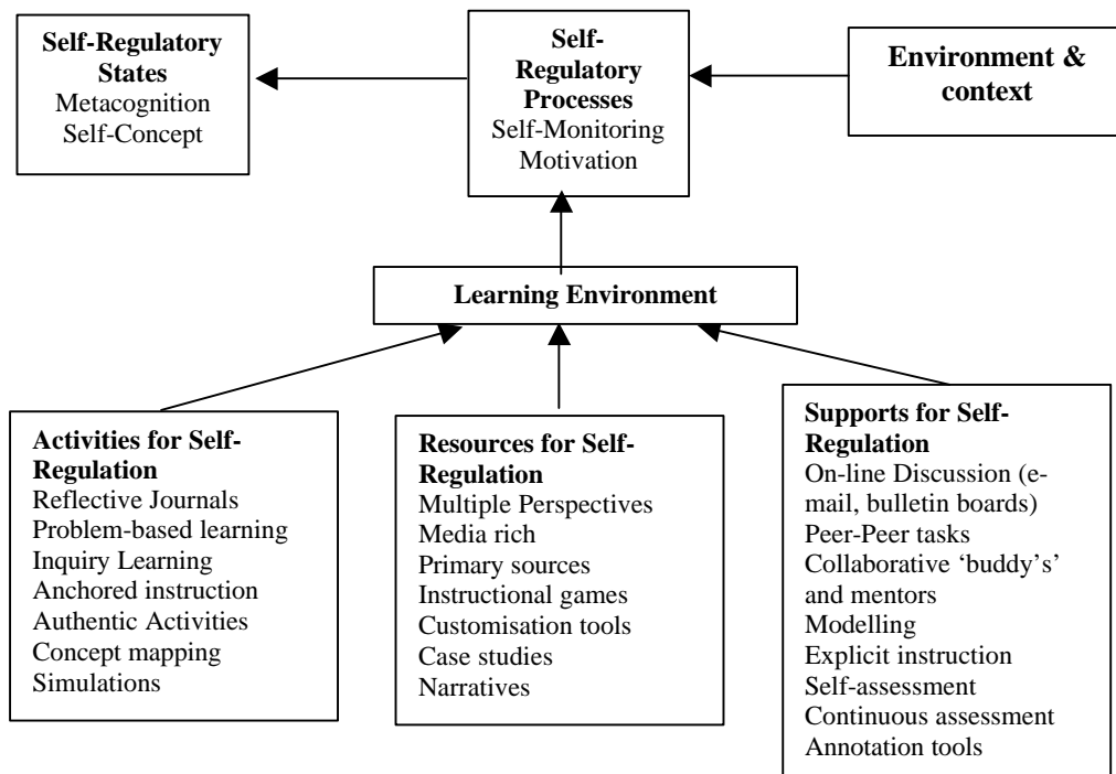
Figure 2 - Self-Regulatory Processes
